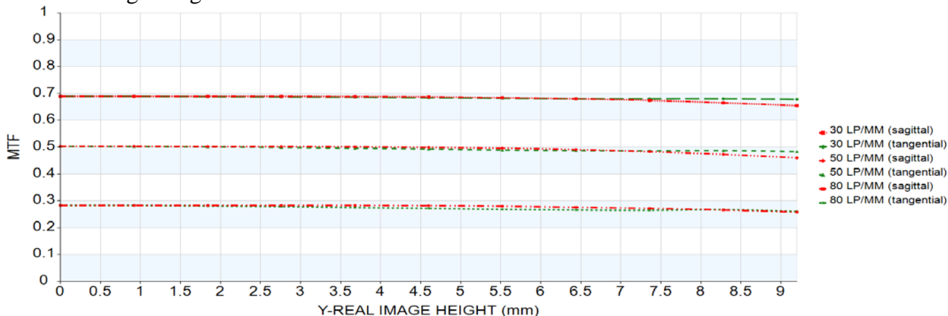
MTF vs Image Height F#13
