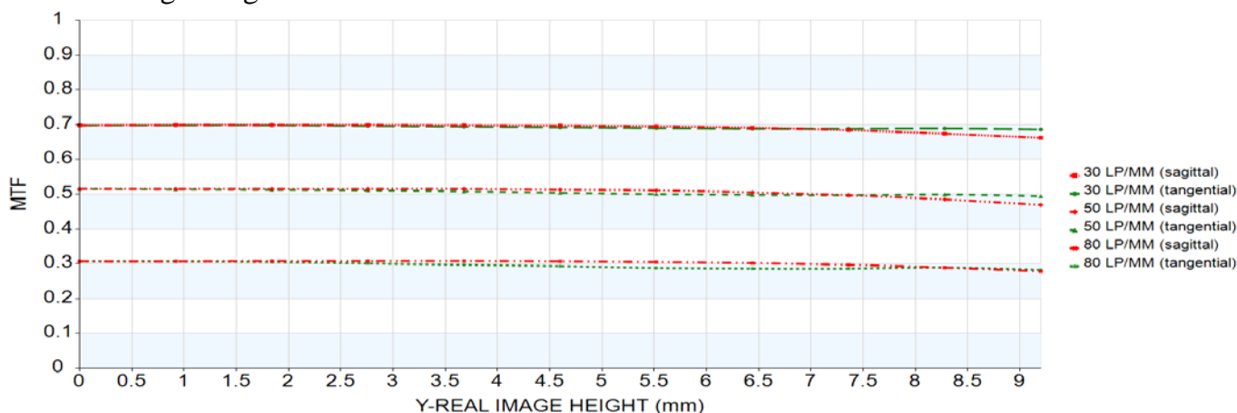
MTF vs Image Height F#12
